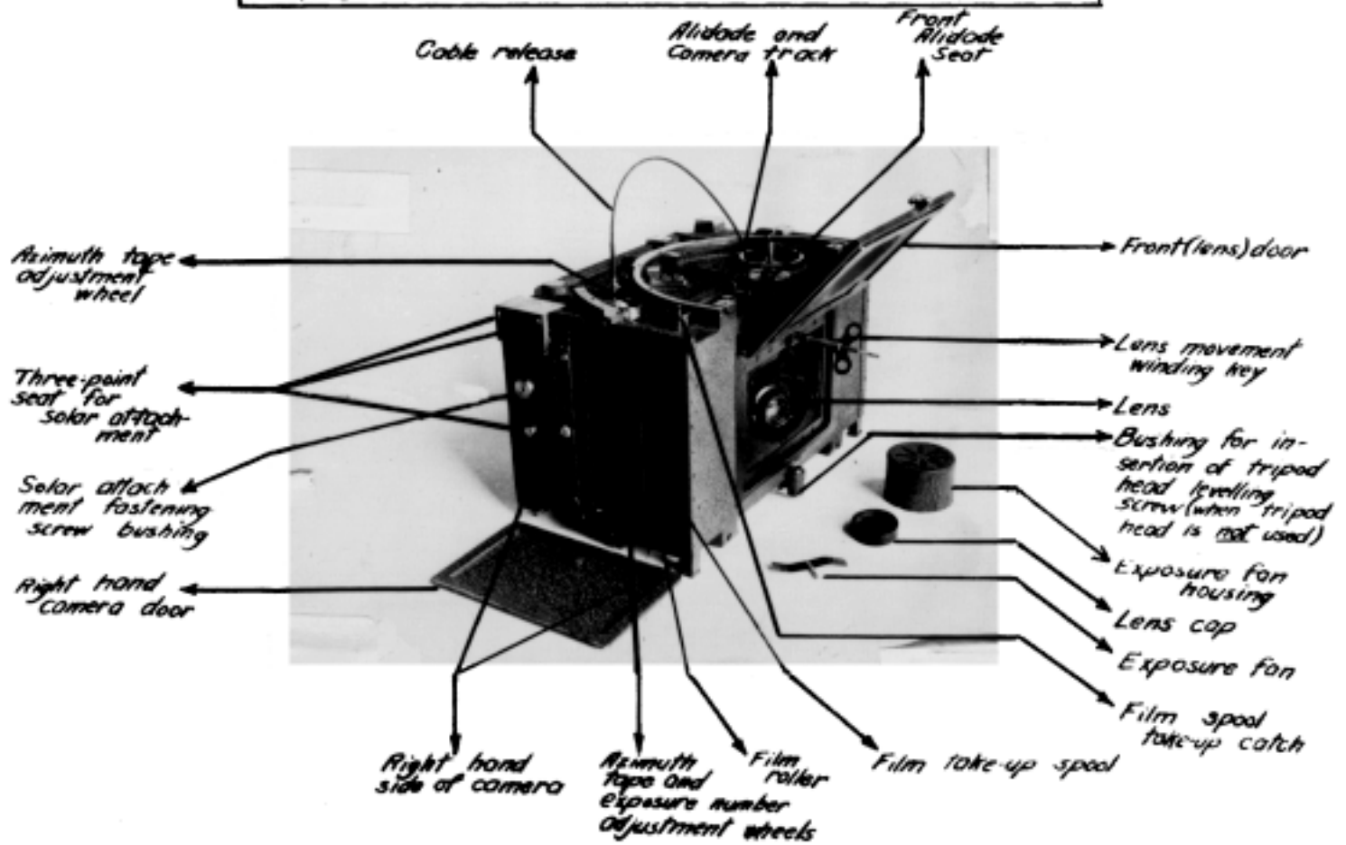
Panoramic Camera in Normal Position
