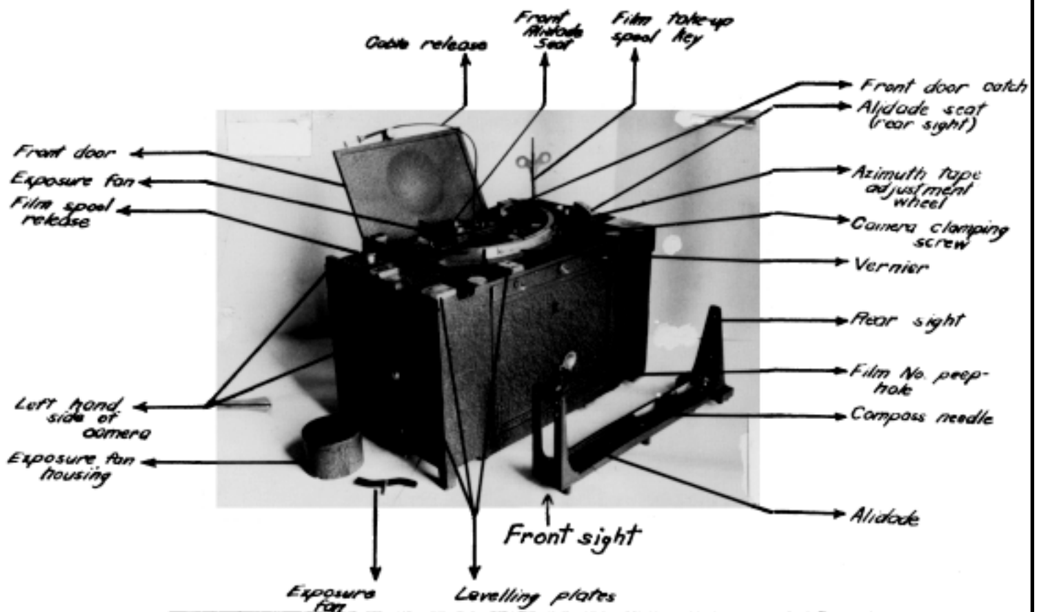
Panoramic Camera in Normal Position
